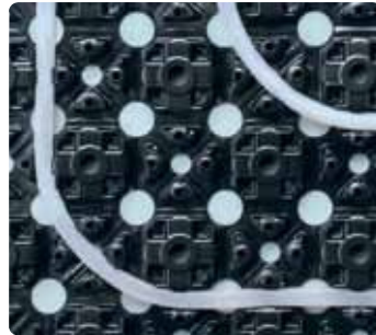
Uponor PE-Xa pipe installed at 90° angle
