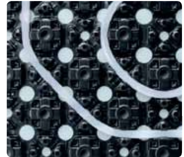
Uponor PE-Xa pipe installed at 45° angles
